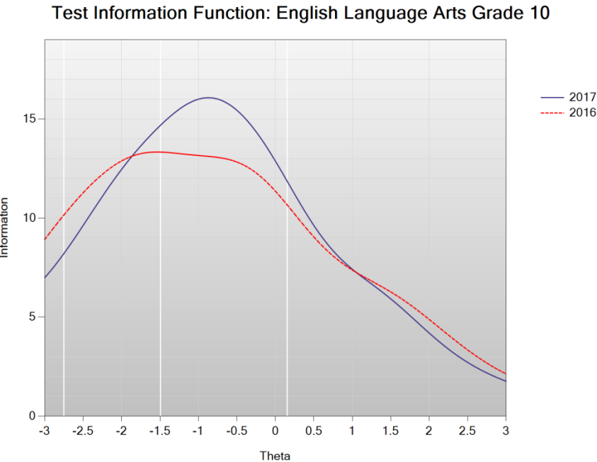
Figure J-2. 2017 Legacy MCAS: Test Information Function – ELA Grade 10
